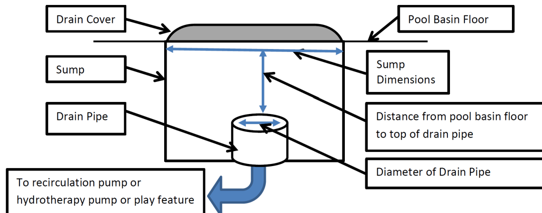
** Example Diagram for Sump Details:
